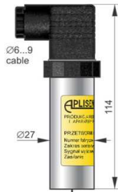
PD type IP65
