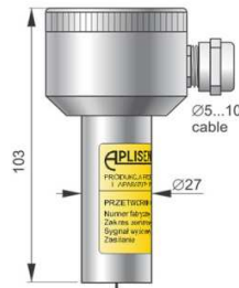
PZ type PZ316 type IP66
