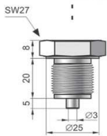
G1/2 type G1/2", Ø3 hole M type M20×1.5, Ø3 hole
